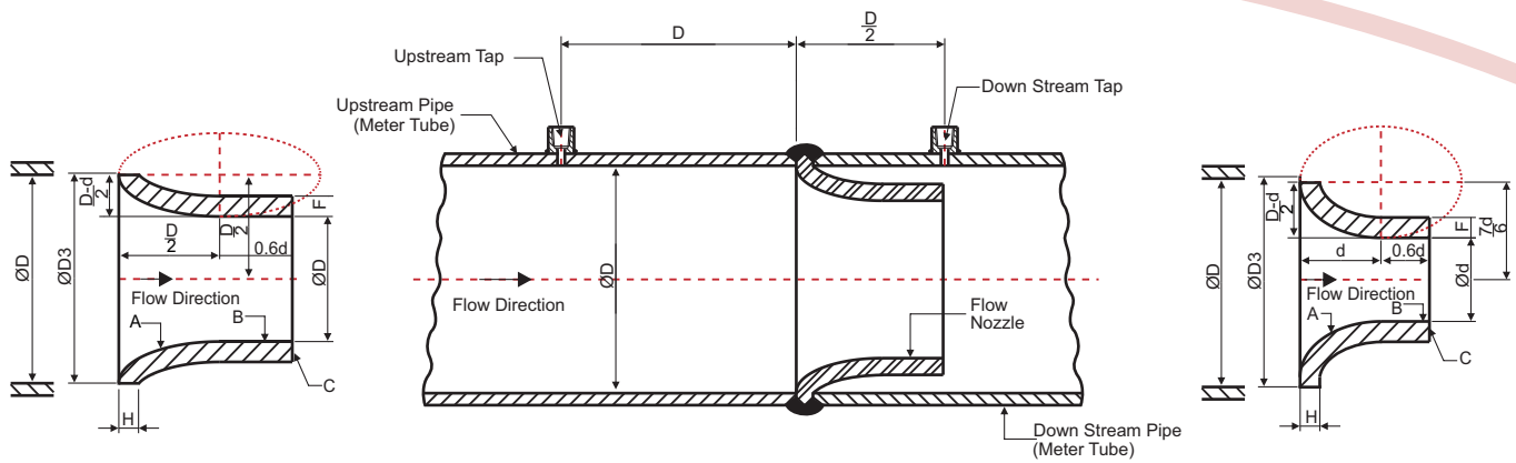
a) LONG RADIUS FLOW NOZZLES - High Beta Ratio 0.25 \geq \beta \geq 0.8 DESIGN STANDARD ISO 5167 / ASME MFC 3M
